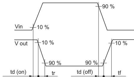
Waveforms
